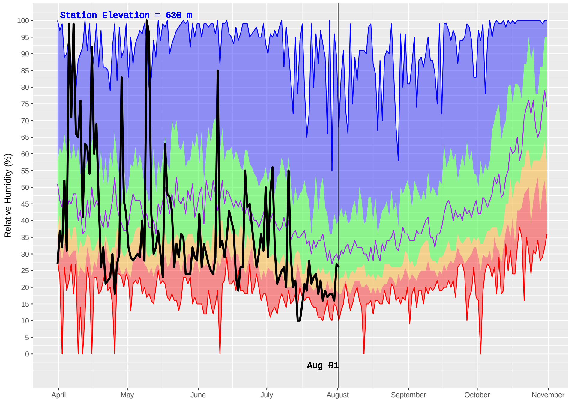
GRAND FORKS (392) : Historical (1981–2016) and Current (2018) Daily Relative Humidity
