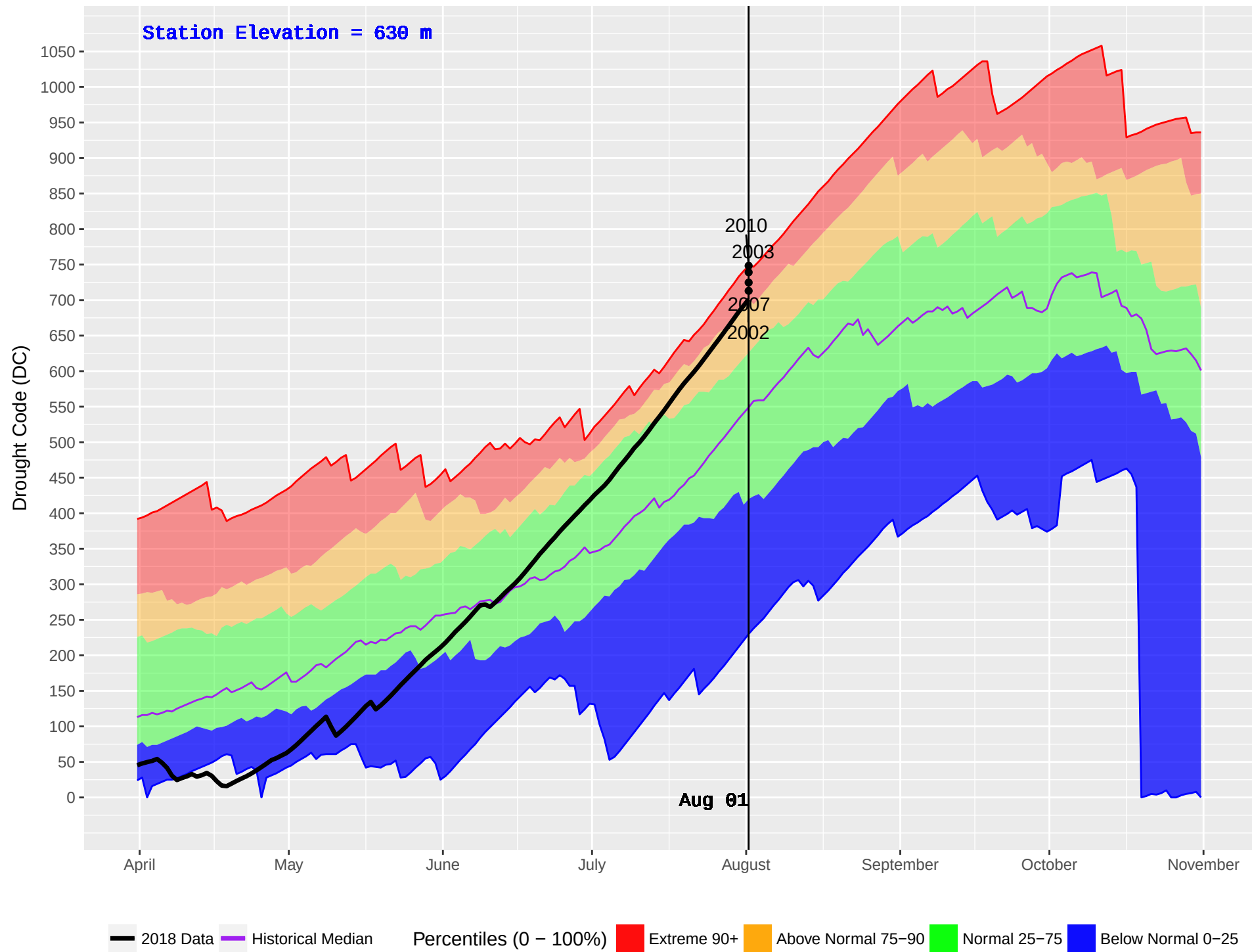
GRAND FORKS (392) : Historical (1981–2016) and Current (2018) Daily Drought Code (DC)
