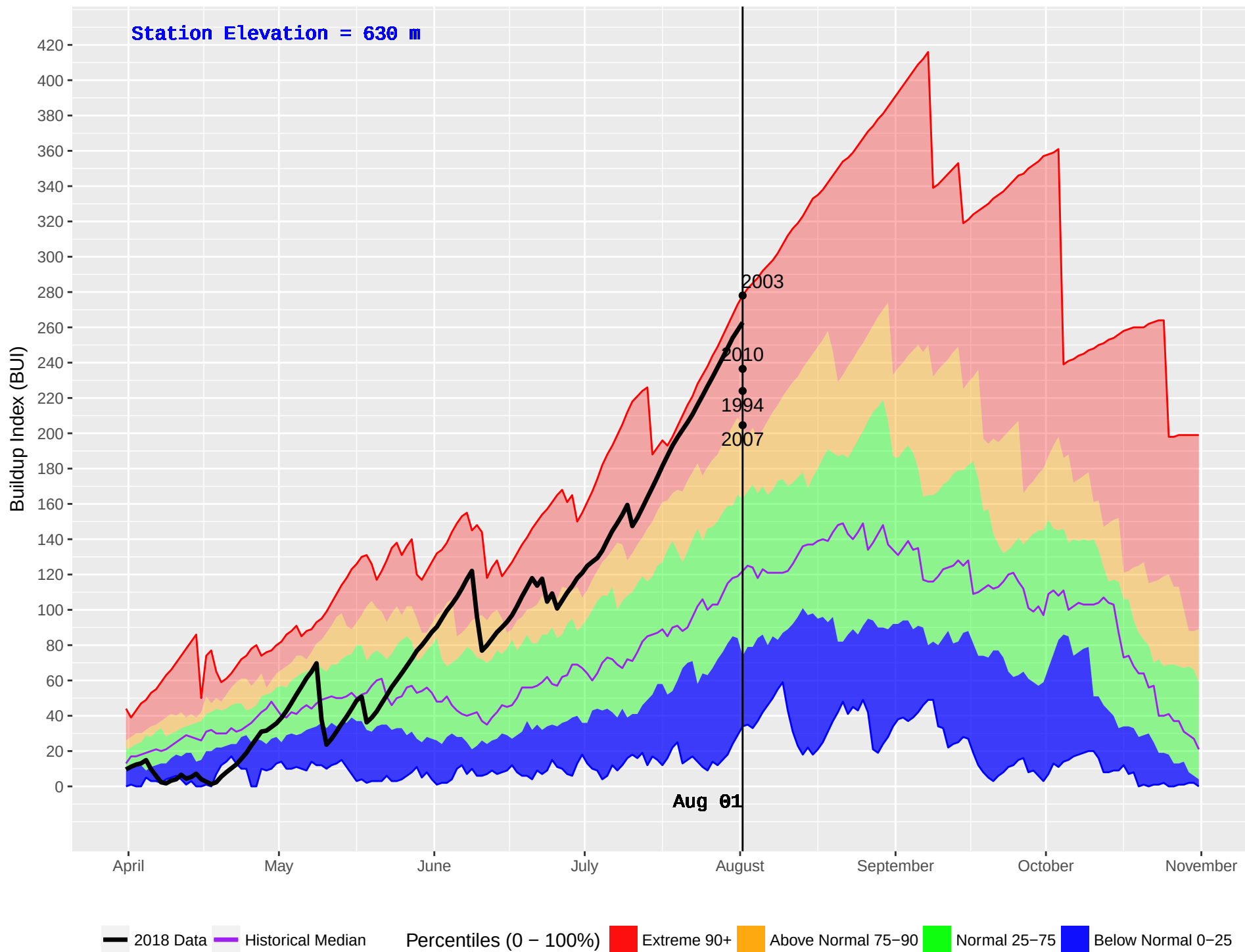
GRAND FORKS (392) : Historical (1981–2016) and Current (2018) Daily Buildup Index (BUI)
